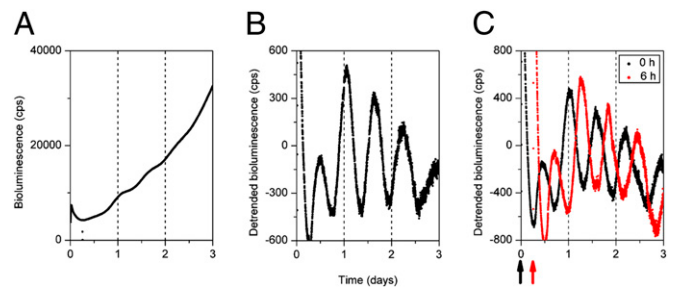
Fig. 1. Rhythmic CCNB1-dGlc expression in rat-1 fibroblasts is synchronized by changing the media. Rat-1 fibroblasts (0.5% confluency) stably expressing CCNB1-dGlc were subcultured in growth media and maintained in a CO 2 incubator. Two days later, the growth media were replaced with recording media and luminescence was recorded. (A) Raw CCNB1-dGlc bioluminescence (counts/s) was measured for 3 days. (B) Detrended CCNB1-dGlc bioluminescence (counts/s) was obtained by subtracting the 14-h moving average from the raw data. A representative example is shown in A and B (from a total of eight dishes). (C) Two days after subculture, the growth media were replaced with recording media in one set of dishes at 0 h (black trace; n = 4 ) and 6 h later in another set of dishes (red trace; n = 4 ). Detrended (subtracted 14-h moving average) CCNB1-dGlc bioluminescence is shown. Arrows indicate the time of media change (luminescence recording start time).
